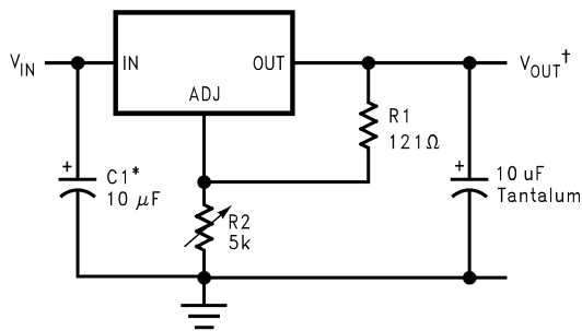
Adjustable @ 5V
