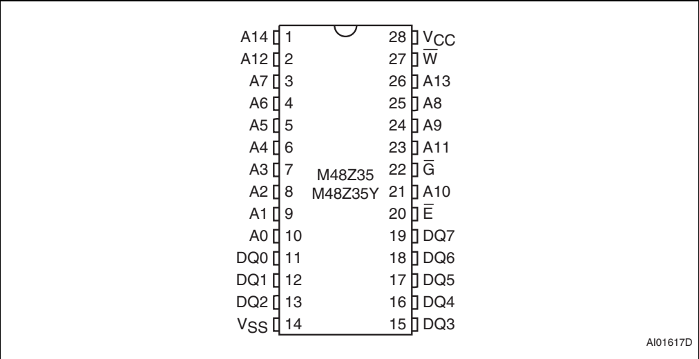
Figure 2. DIP connections
