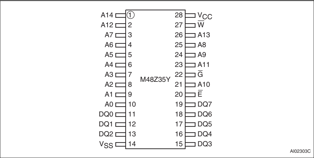
Figure 3. SOIC connections
