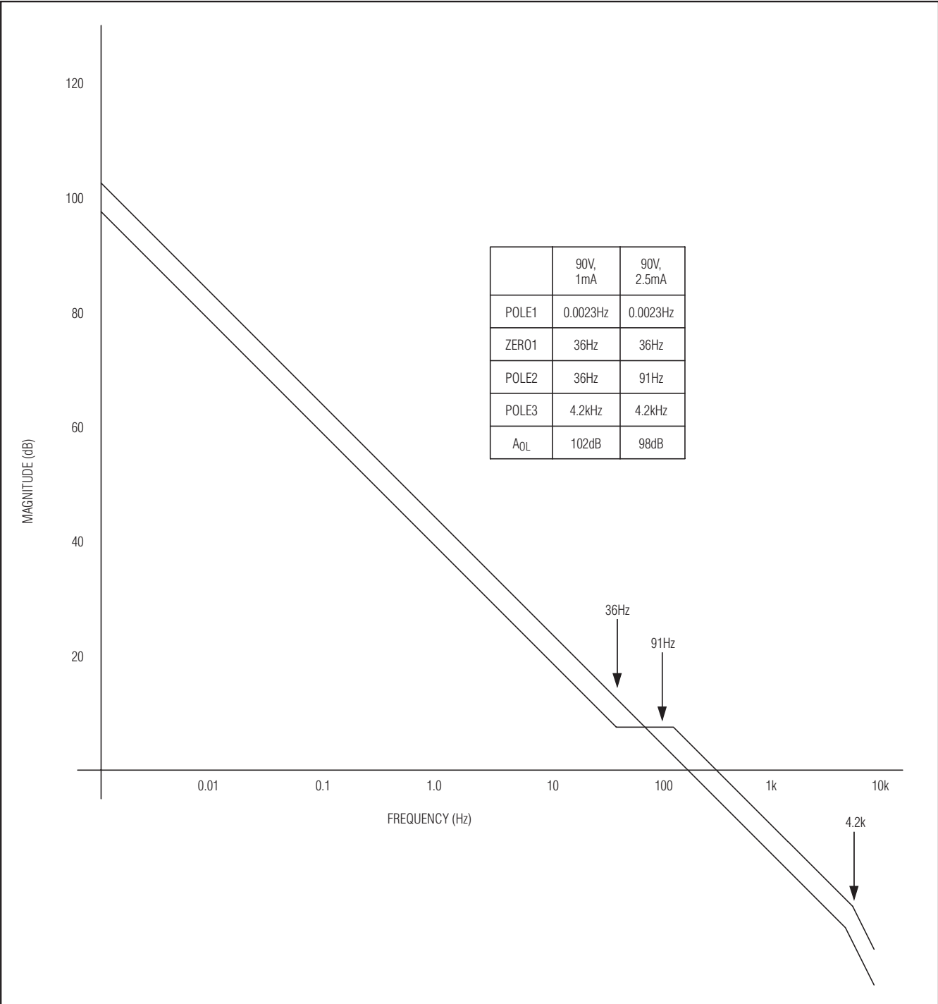
Figure 6. Loop Response
