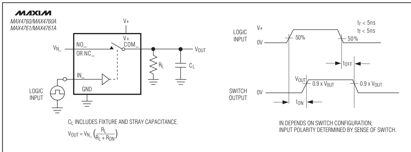
Figure 2. Switching Time
