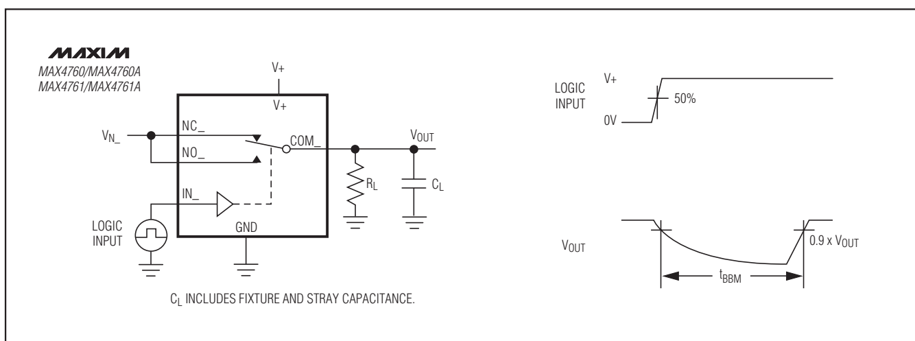
Figure 3. Break-Before-Make Interval
