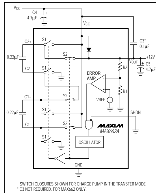
Figure 1. Block Diagram
