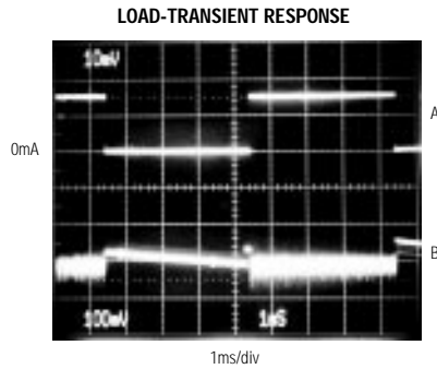
A: OUTPUT CURRENT, 20mA/div, I_{OUT} = 0\text{mA} to 30mA B: OUTPUT VOLTAGE RIPPLE, 100mV/div, V_{CC} = 5.0\text{V}
