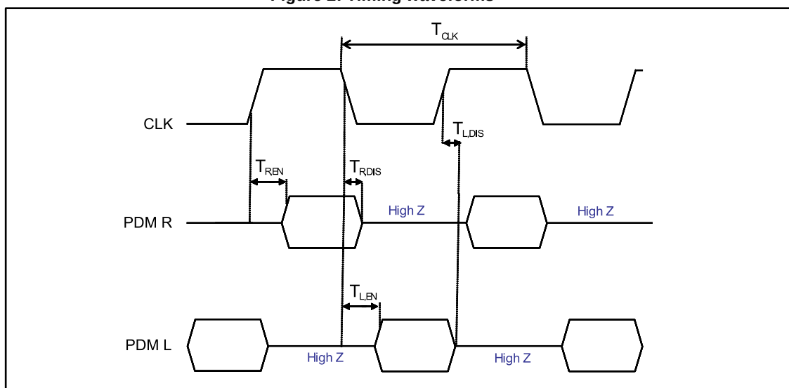
Figure 2: Timing waveforms
