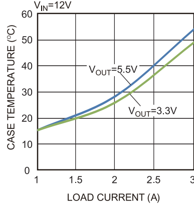
Case Temperature Rise vs. I_{OUT}
