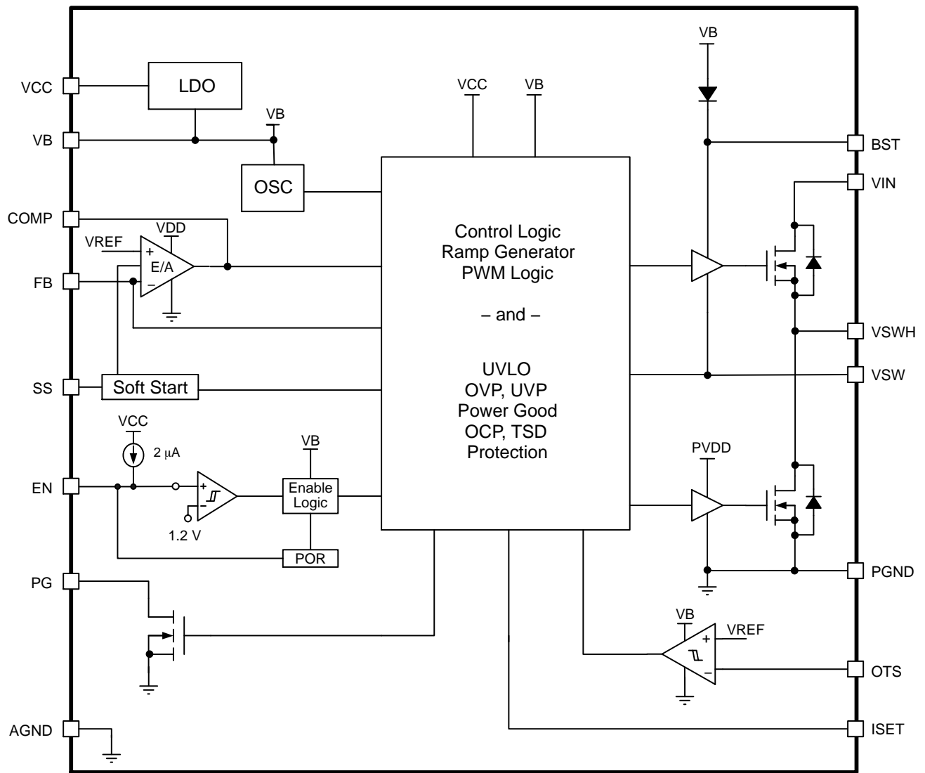
Figure 1. NCP3230 Block Diagram
