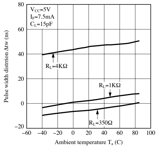
Fig.14 Distortion of Pulse width vs. Ambient Temperature
