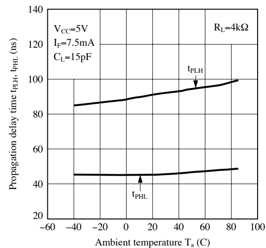
Fig.12-c Propagation Delay Time vs. Ambient Temperature
