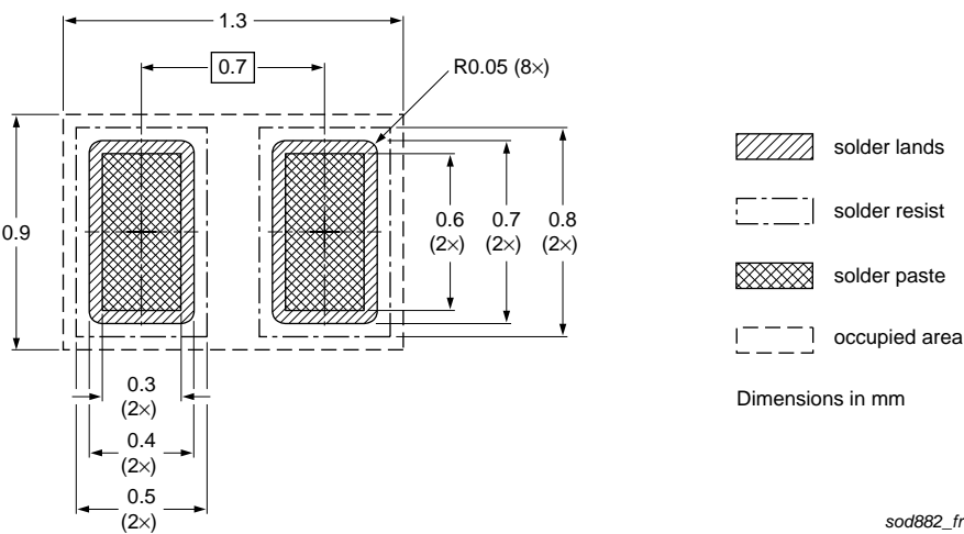
Fig 16. Reflow soldering footprint PESD5V0V1BL (SOD882)
