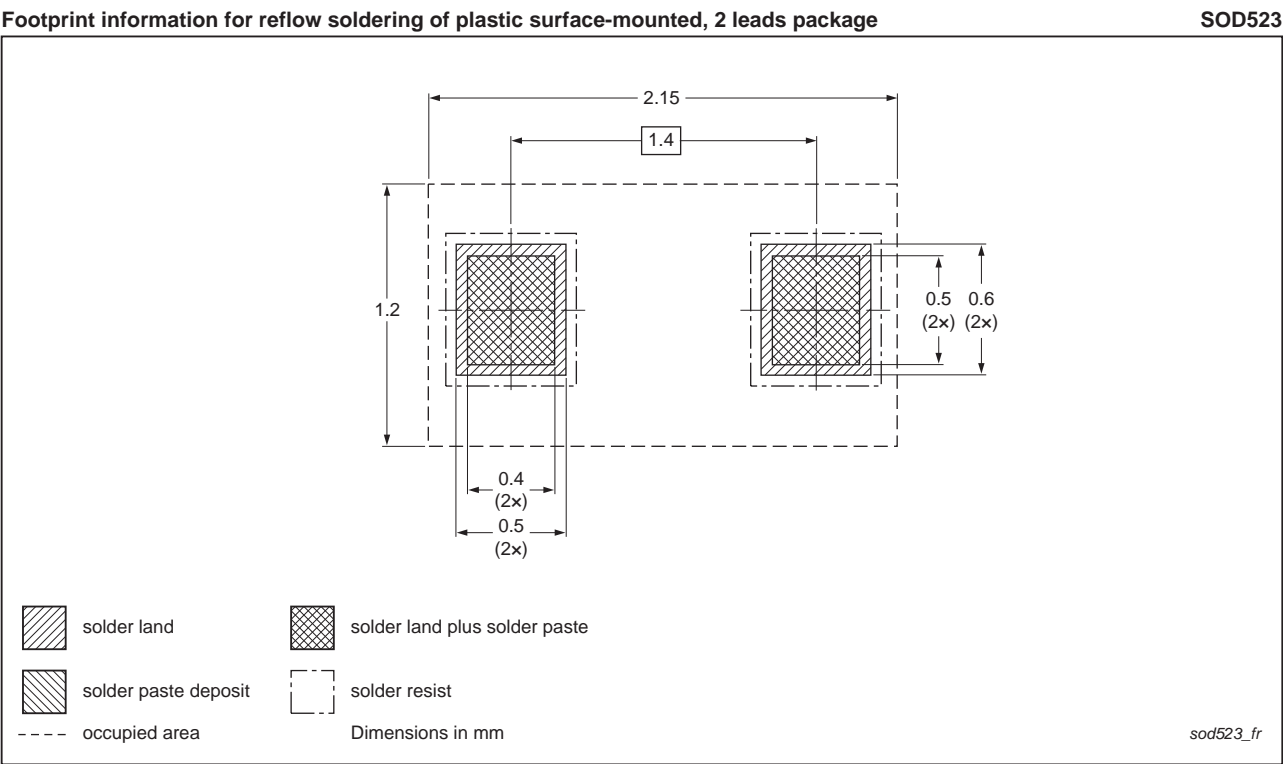
Fig 15. Reflow soldering footprint PESD5V0V1BB (SOD523/SC-79)
