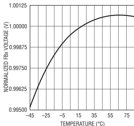
Normalized FBx Reference vs Temperature
