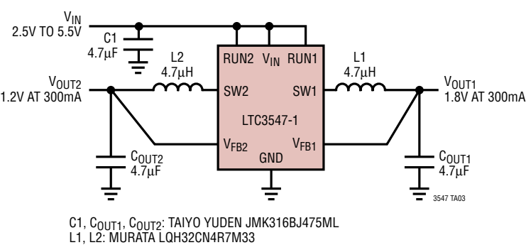
1.8V/1.2V Dual 300mA Buck Converter
