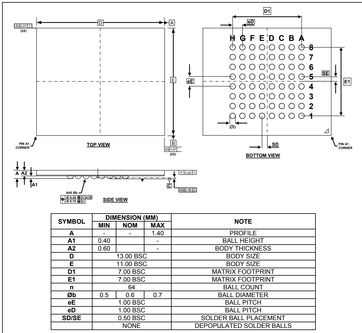
Figure 9-2 LFBGA 64-ball 11x13mm
