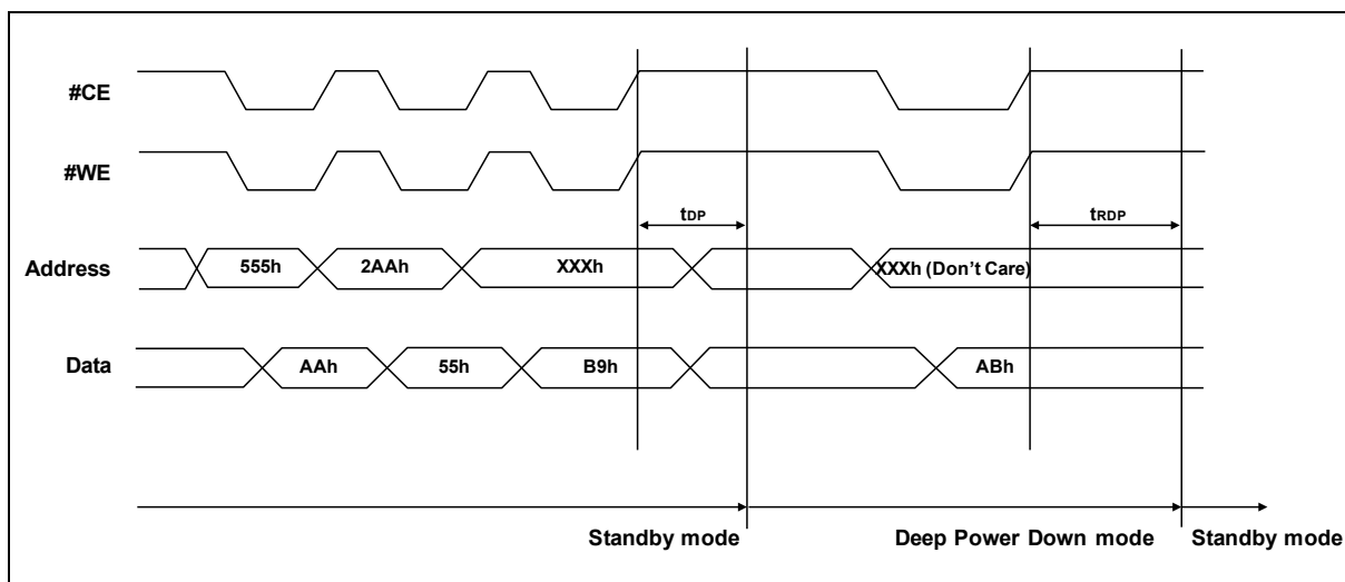
Figure 8-25 Deep Power Down mode Waveform
