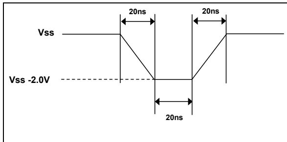
Figure 8-1 Maximum Negative Overshoot
