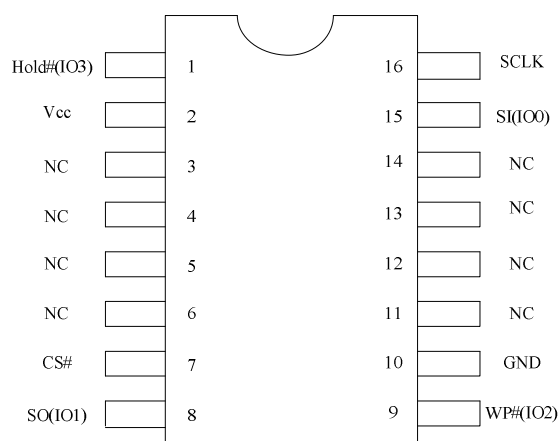
16-Pin SOIC
