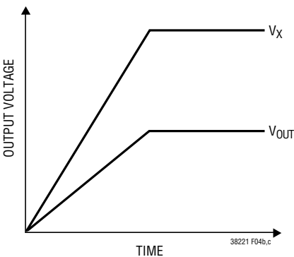
(4c) Ratiometric Tracking
