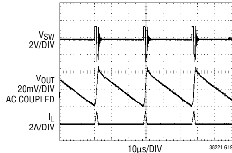
FIGURE 10 CIRCUIT V_{IN} = 3.3\text{V} V_{OUT} = 1.8\text{V} , 100mA
