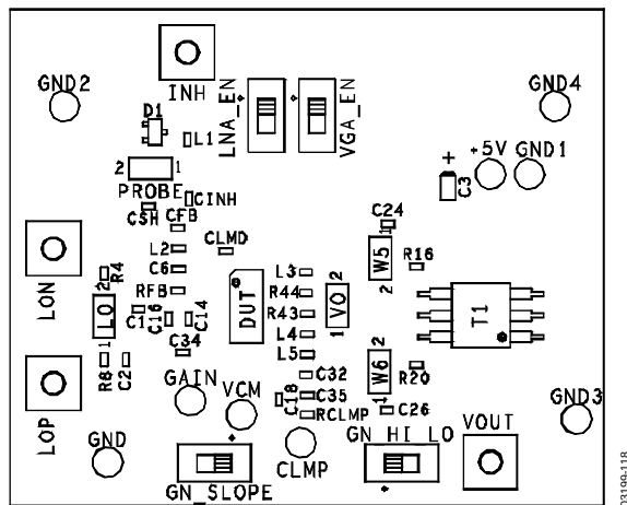
Figure 98. AD8331-EVALZ Assembly
