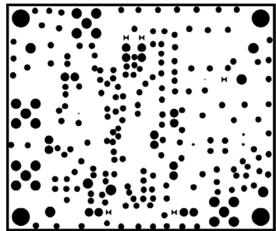
Figure 102. Power Plane
