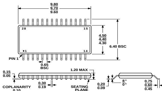
Figure 122. 28-Lead Thin Shrink Small Outline Package (TSSOP) (RU-28)
