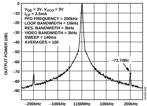
Figure 8. Reference Spurs at 1150 MHz (200 kHz Channel Spacing, 10 kHz Loop Bandwidth)
