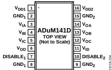
Figure 9. ADuM141D Pin Configuration
