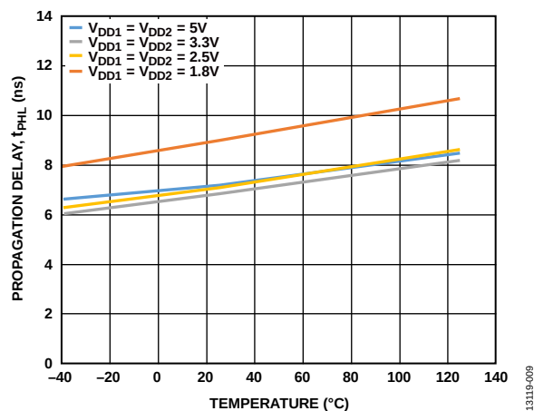
Figure 20. Propagation Delay, t_{PHL} vs. Temperature at Various Voltages
