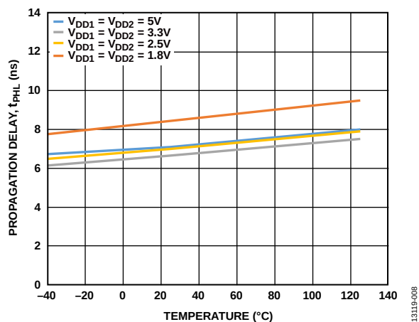
Figure 19. Propagation Delay, t_{PLH} vs. Temperature at Various Voltages
