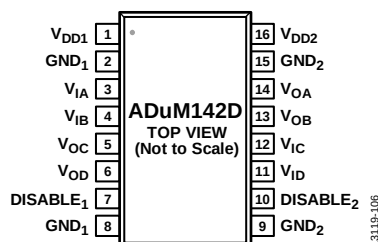
Figure 11. ADuM142D Pin Configuration
