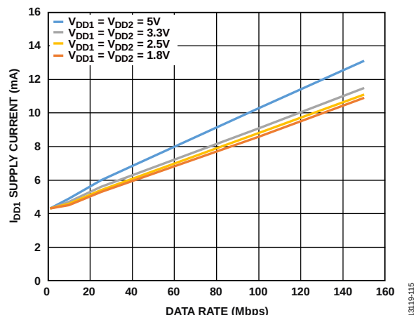
Figure 17. ADuM142D/ADuM142E I_{DD1} Supply Current vs. Data Rate at Various Voltages
