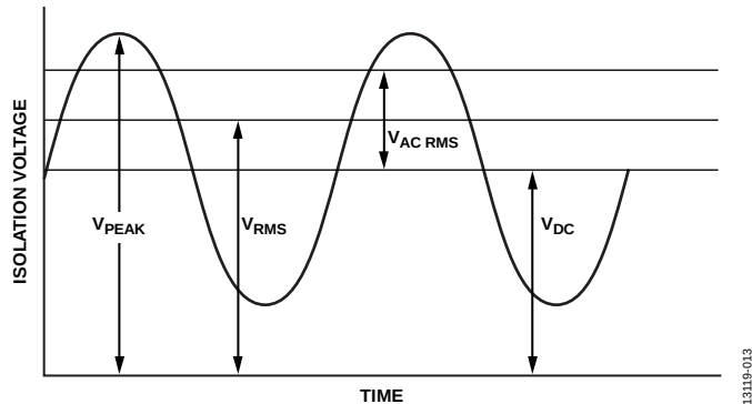
Figure 26. Critical Voltage Example
