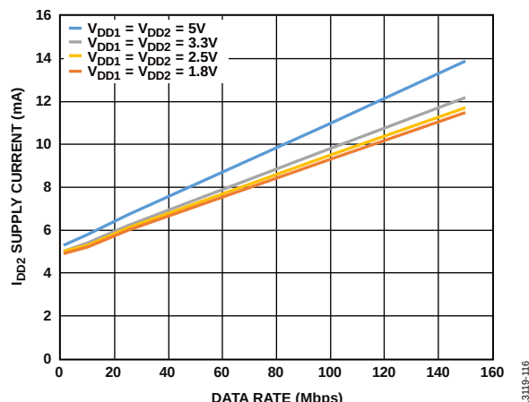
Figure 18. ADuM142D/ADuM142E I_{DD2} Supply Current vs. Data Rate at Various Voltages
