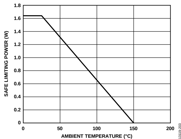
Figure 6. Thermal Derating Curve for RQ-16 [QSOP] Package, Dependence of Safety Limiting Values with Ambient Temperature per DIN V VDE V 0884-10
