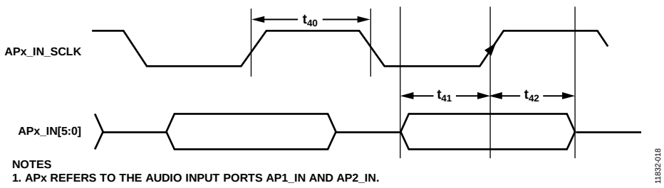
Figure 14. DSD Input Timing
