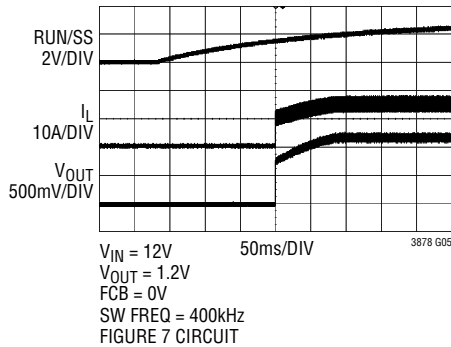
Normal Start-Up, RUN/SS Release from Zero
