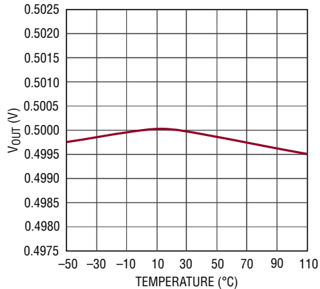
Regulated Output vs Temperature
