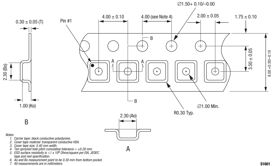
Figure 11. CLA4603-085LF Tape and Reel Dimensions
