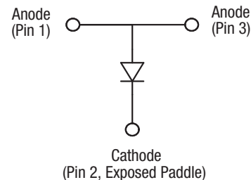
Figure 1. CLA4603-085LF Block Diagram
