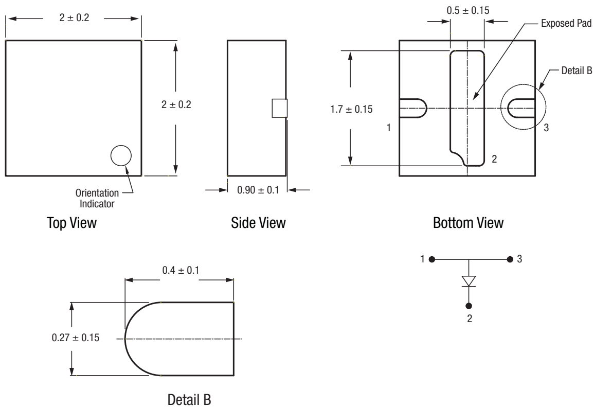
Figure 10. CLA4603-085LF QFN Package Dimension Drawing
