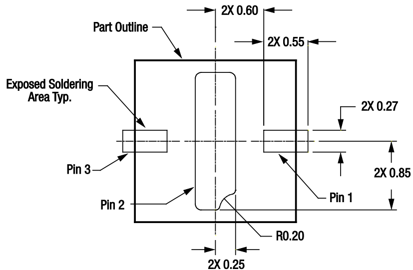
Figure 7. CLA4605-085LF PCB Layout Footprint
