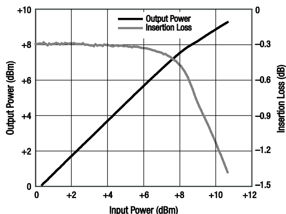
Figure 4. Output Power and Insertion Loss vs Input Power ( f = 2.5\text{ GHz} )
