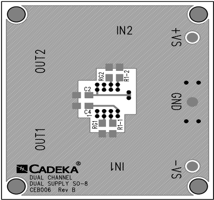
Figure 10. CEB006 Top View
