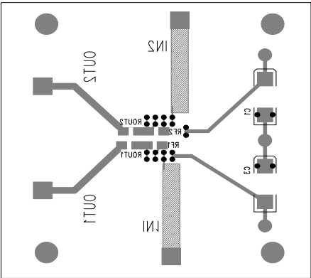
Figure 11. CEB006 Bottom View
