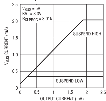
V_{BUS} Current vs V_{OUT} Current in Suspend
