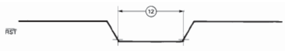
Figure 1. Reset Waveform
