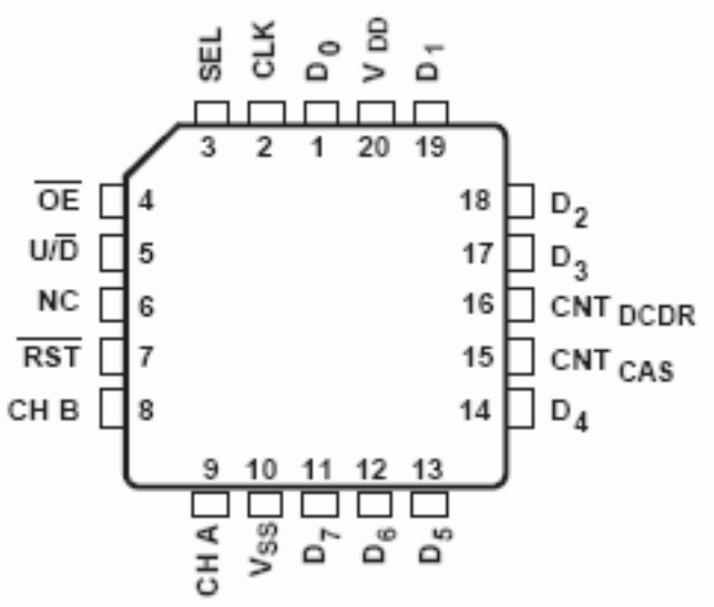
PINOUT D
