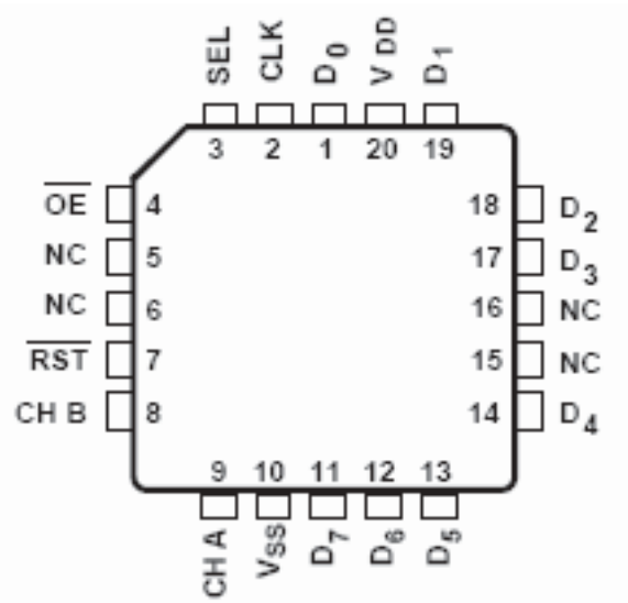
PINOUT C
