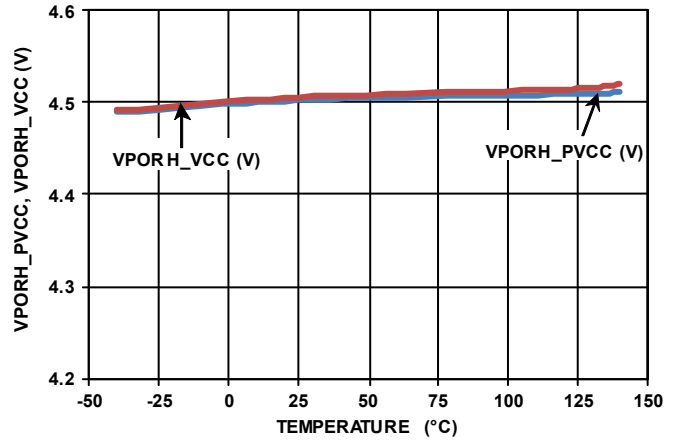
FIGURE 42. PVCC/VCC POR RISING THRESHOLD vs TEMPERATURE
