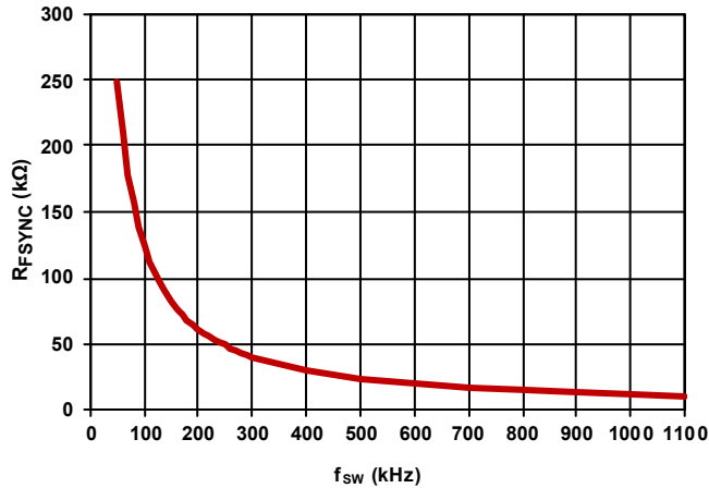
FIGURE 55. f_{SW} vs R_F
