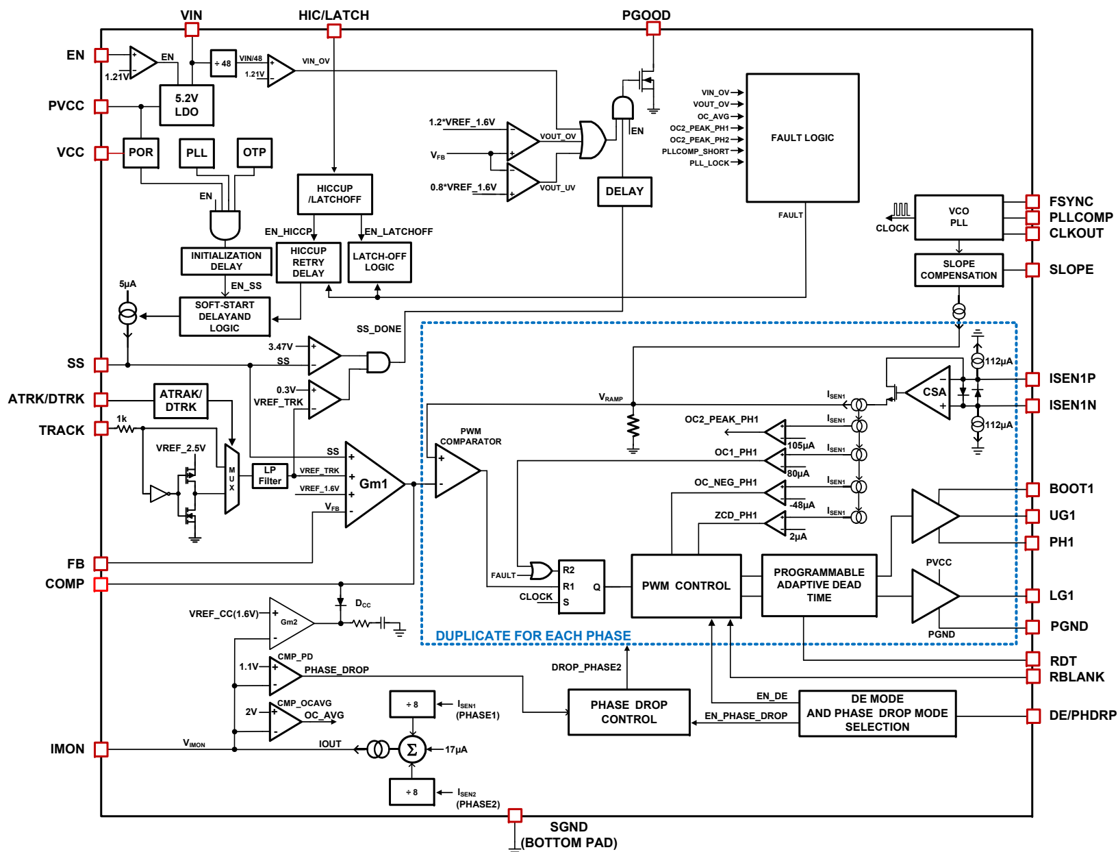
FIGURE 3. BLOCK DIAGRAM
