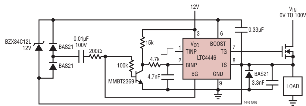
LTC4446 Fast Turn-On/Turn-Off DC Switch
