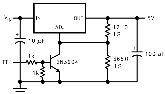
Figure 23. Adjustable @ 5V
