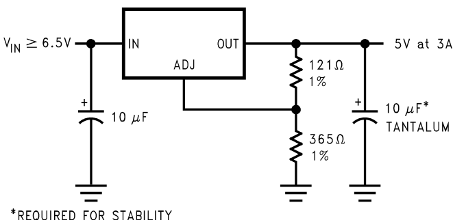
Figure 23. Adjustable @ 5V
