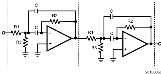
FIGURE 4. Active Filter
