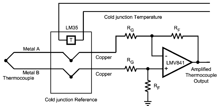
FIGURE 9. Thermocouple Amplifier
