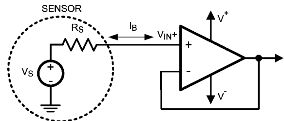
FIGURE 7. High Impedance Sensor Interface
