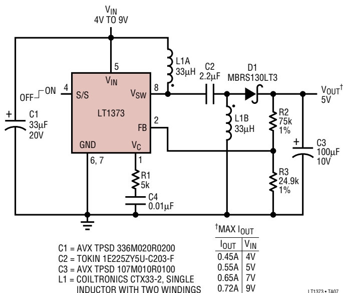
Two Li-Ion Cells to 5V SEPIC Converter
