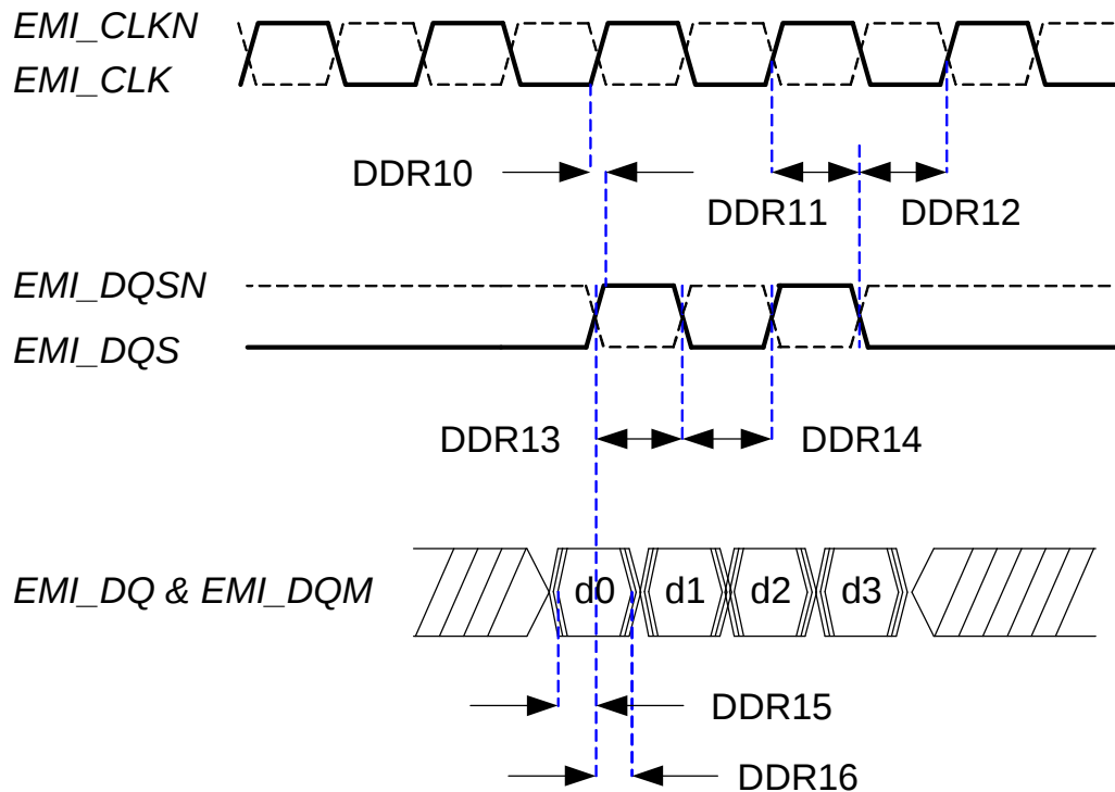
Figure 6. DDR Output AC Timing
