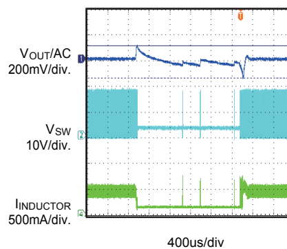
Transient Response I_{OUT}=0mA-50mA
