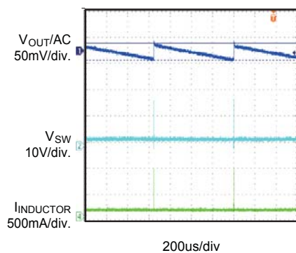
PFM Operation No Load
