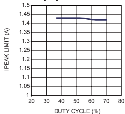
SW peak current limit vs. Duty Cycle
