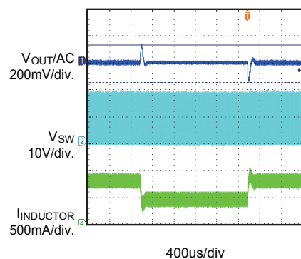
Transient Response I_{OUT}=50mA-100mA
