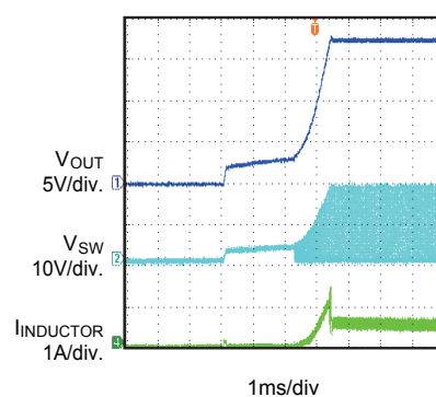
Startup I_{OUT}=100mA
