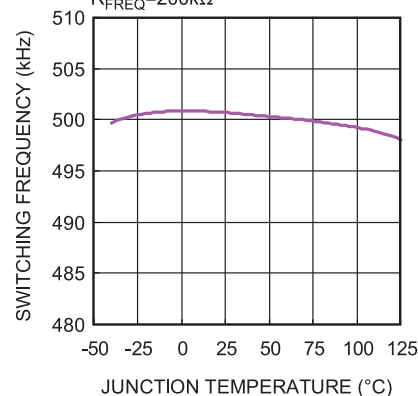
Frequency vs. Junction Temperature R_{FREQ} = 200k\Omega
