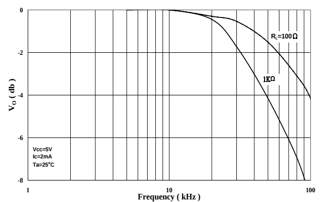
Figure 18. Frequency Response
