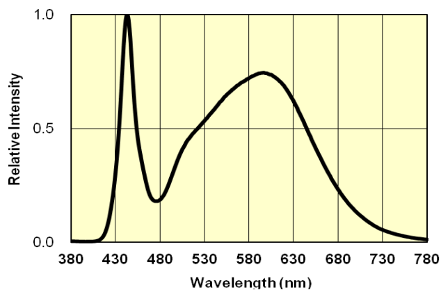
Fig.1 Typical Spectrum
