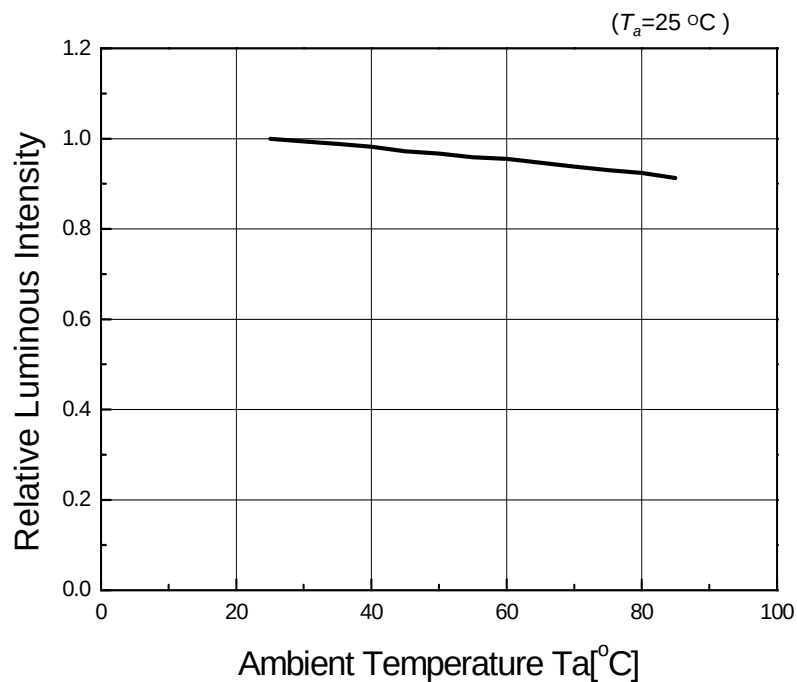
Ambient Temperature vs. Relative Intensity
