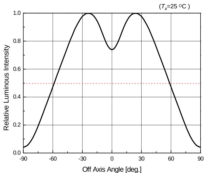
Radiation Diagram
