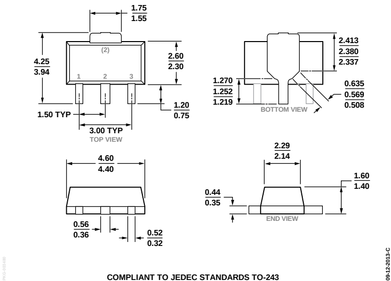
Figure 22. 3-Lead Small Outline Transistor Package [SOT-89] (RK-3) Dimensions shown in millimeters
