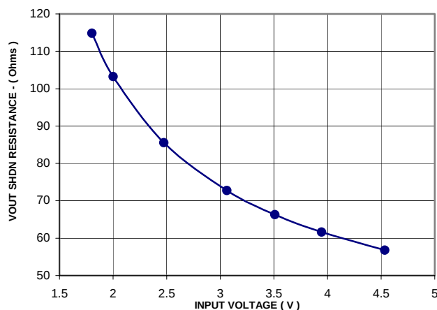
Figure 13 – V OUT Shutdown Resistance vs. Input Voltage; T_A = 25^\circ\text{C} , C_1 = 0.22\mu\text{F} , C_2, C_3, C_4 = 4.7\mu\text{F} , C_{\text{FILT}} = 0.1\mu\text{F}
