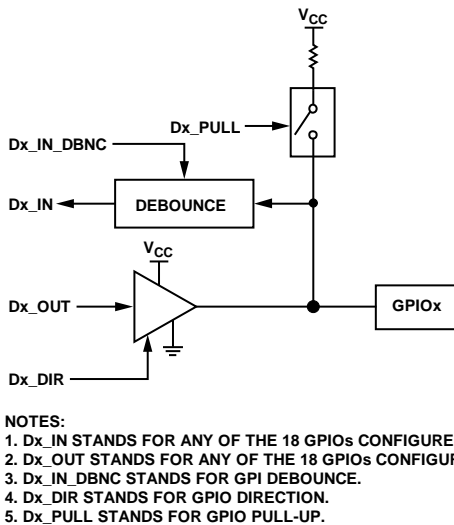
Figure 14. Typical GPIO Block
