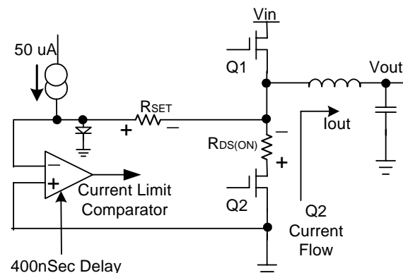
Figure 3 – Phase 1 \bar{C} Current Limit
