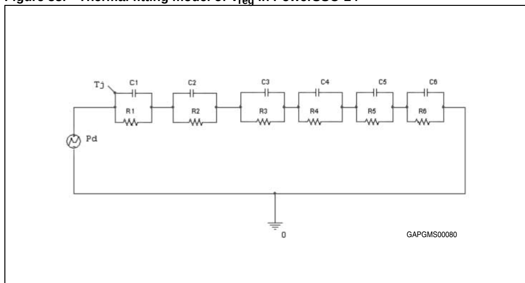
Figure 38. Thermal fitting model of V_{reg} in PowerSSO-24
