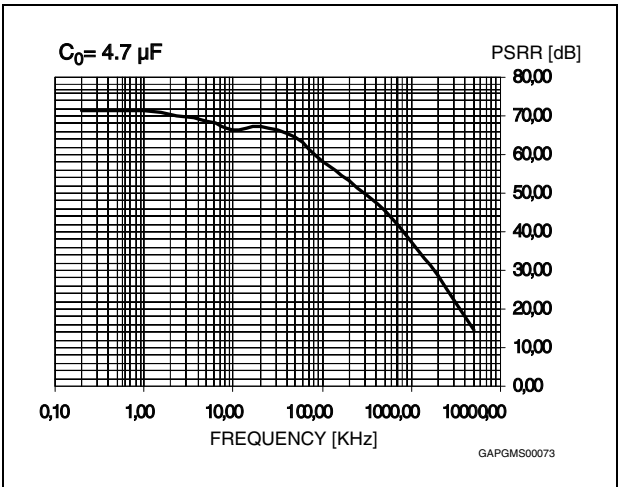
Figure 23. PSRR
