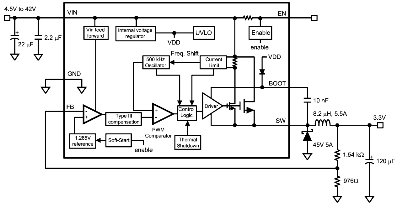
FIGURE 1. 3.3V V_{\text{OUT}} , 3A
