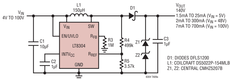
4V to 100V IN /140V OUT Boost Converter
