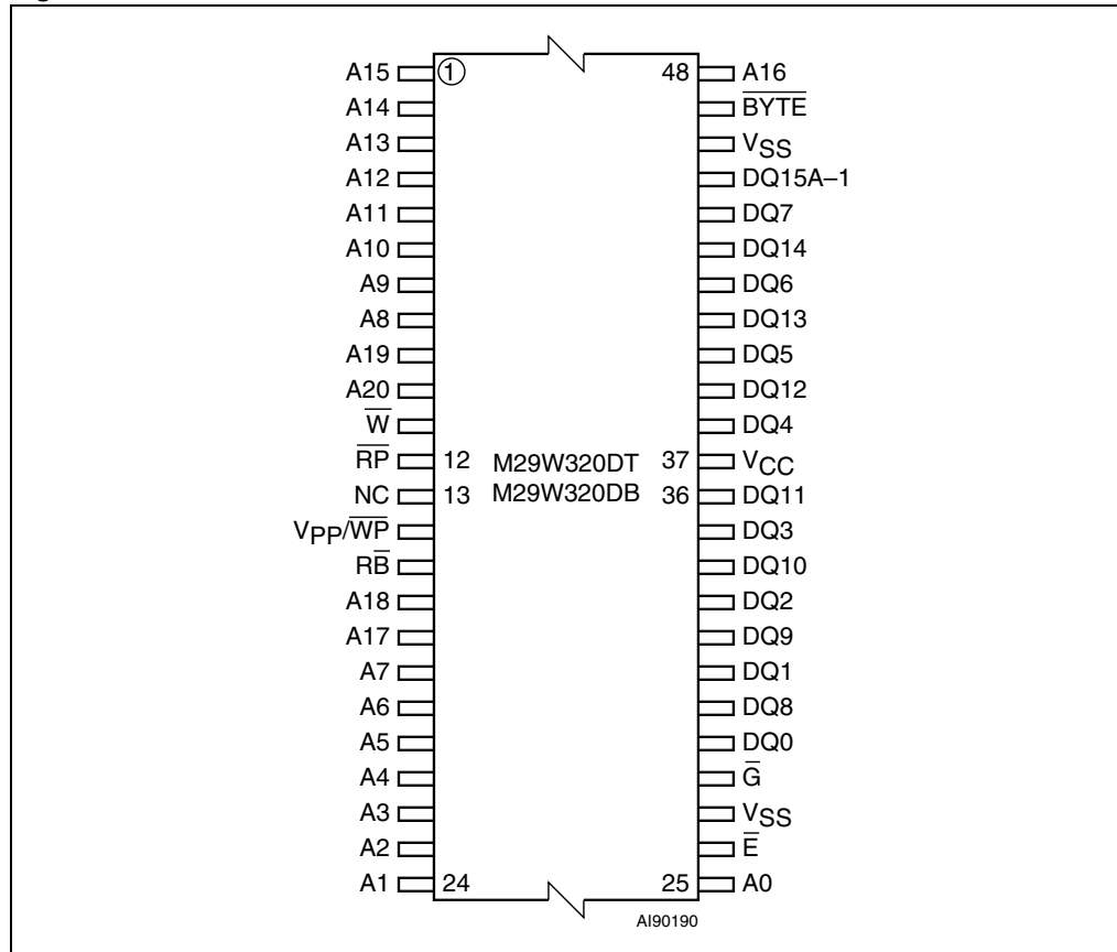
Figure 2. TSOP Connections
