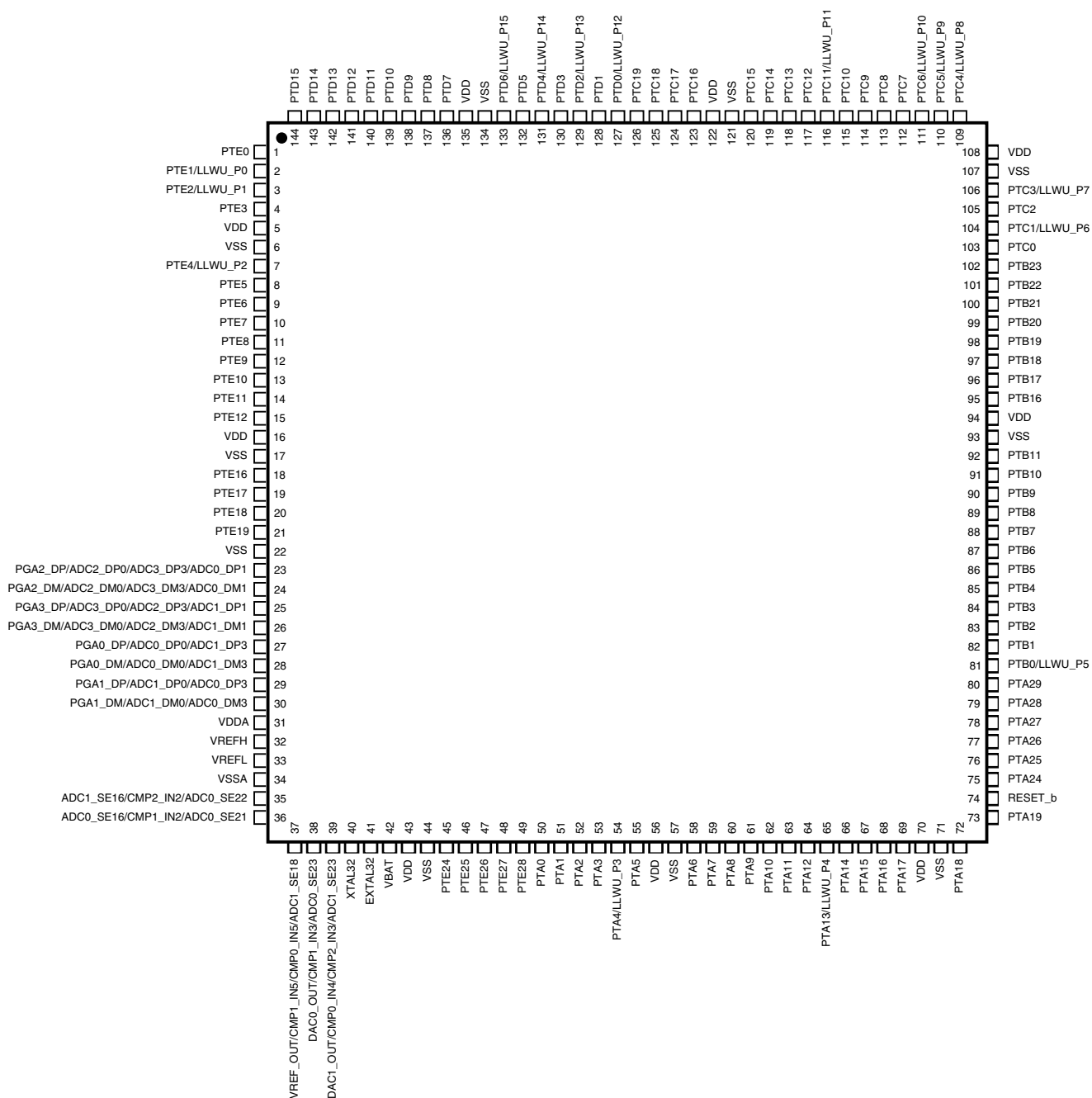
Figure 37. K10 144 LQFP Pinout Diagram
