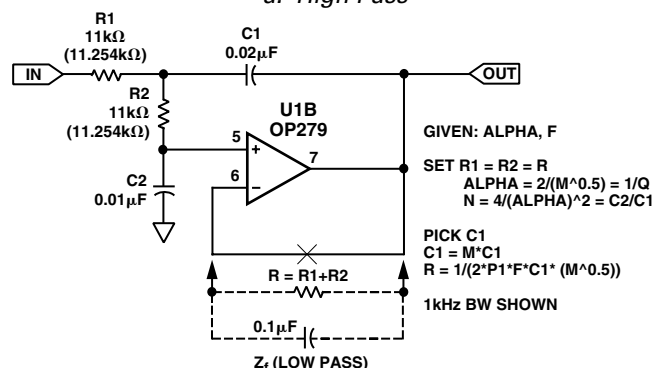
Figure 14. Two-Pole Unity-Gain Sallen Key HP/LP Filters
