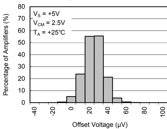
Offset Voltage Production Distribution at +5V
