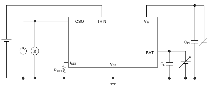
6) Test Circuit ⑥
