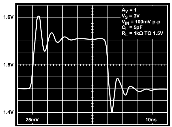
Figure 34. 100 mV Pulse Response, V_S = 3V
